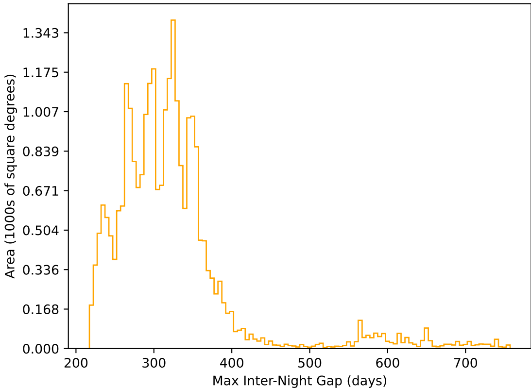
roll_pause_mjdp0_v3.4_10yrs All sky r band: Max Inter-Night Gap
