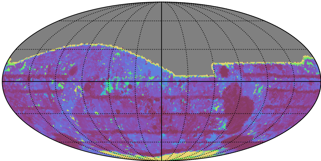
roll_pause_mjdp0_v3.4_10yrs All sky i band: Max Inter-Night Gap
