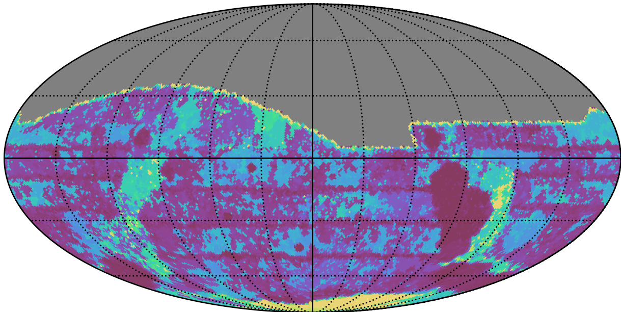
roll_pause_mjdp0_v3.4_10yrs All sky g band: Max Inter-Night Gap
