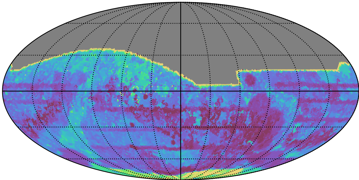
roll_pause_mjdp0_v3.4_10yrs All sky all bands: Max Inter-Night Gap
