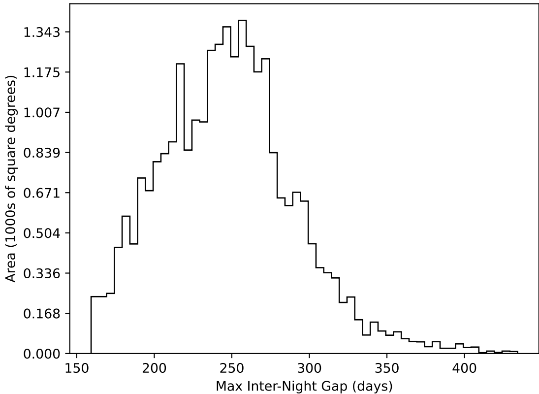
roll_pause_mjdp0_v3.4_10yrs All sky all bands: Max Inter-Night Gap
