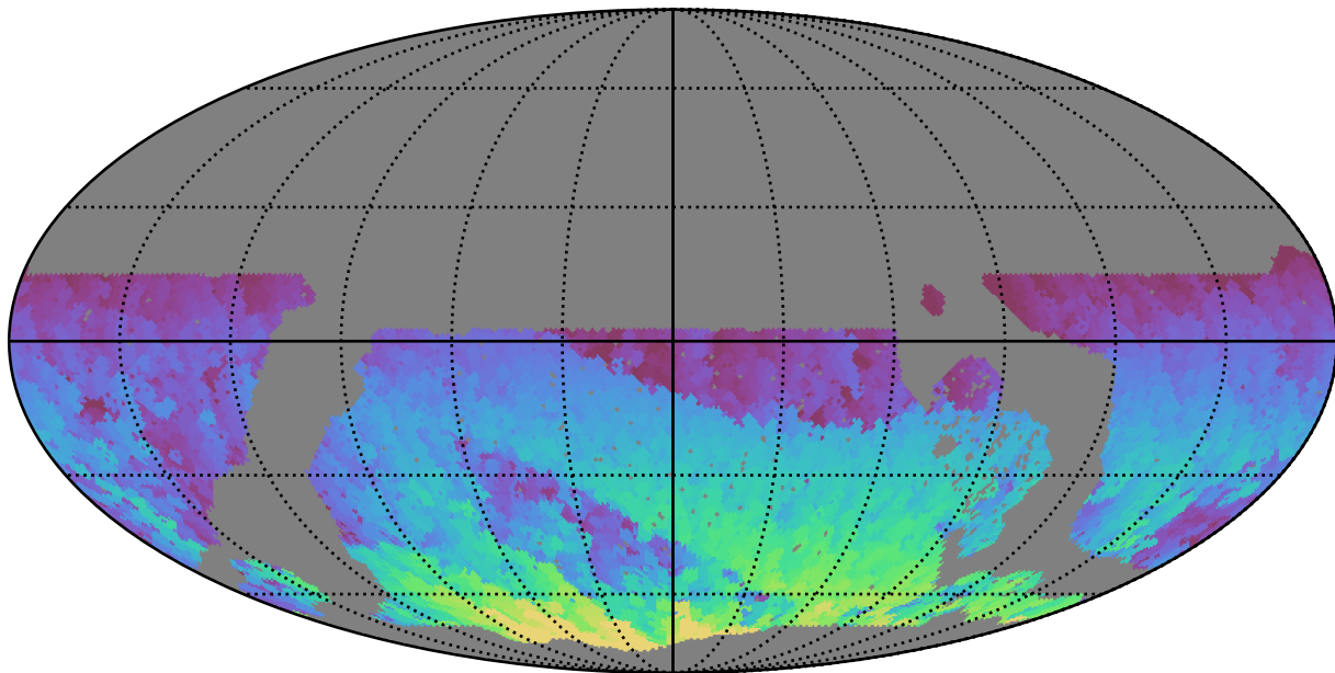
roll_pause_mjdp0_v3.4_10yrs WFD z band: Max HA
