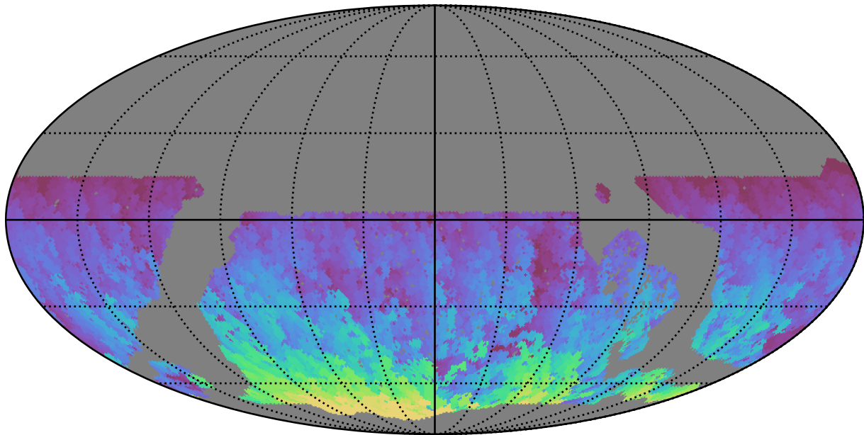
roll_pause_mjdp0_v3.4_10yrs WFD y band: Max HA
