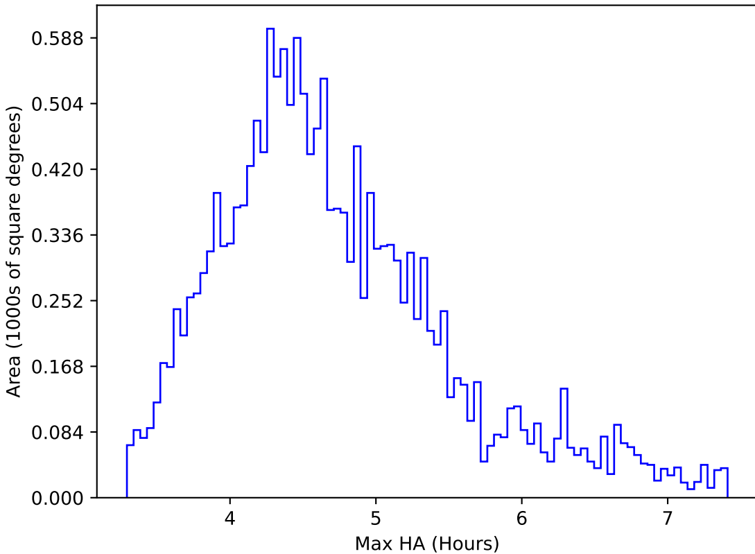
roll_pause_mjdp0_v3.4_10yrs WFD y band: Max HA
