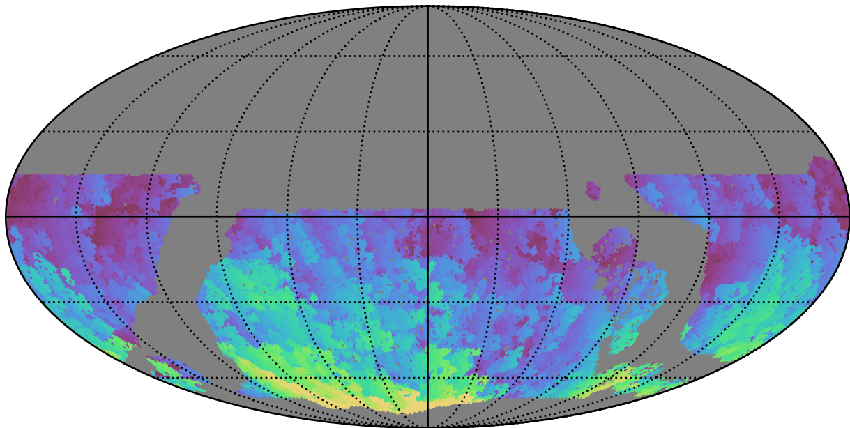
roll_pause_mjdp0_v3.4_10yrs WFD u band: Max HA
