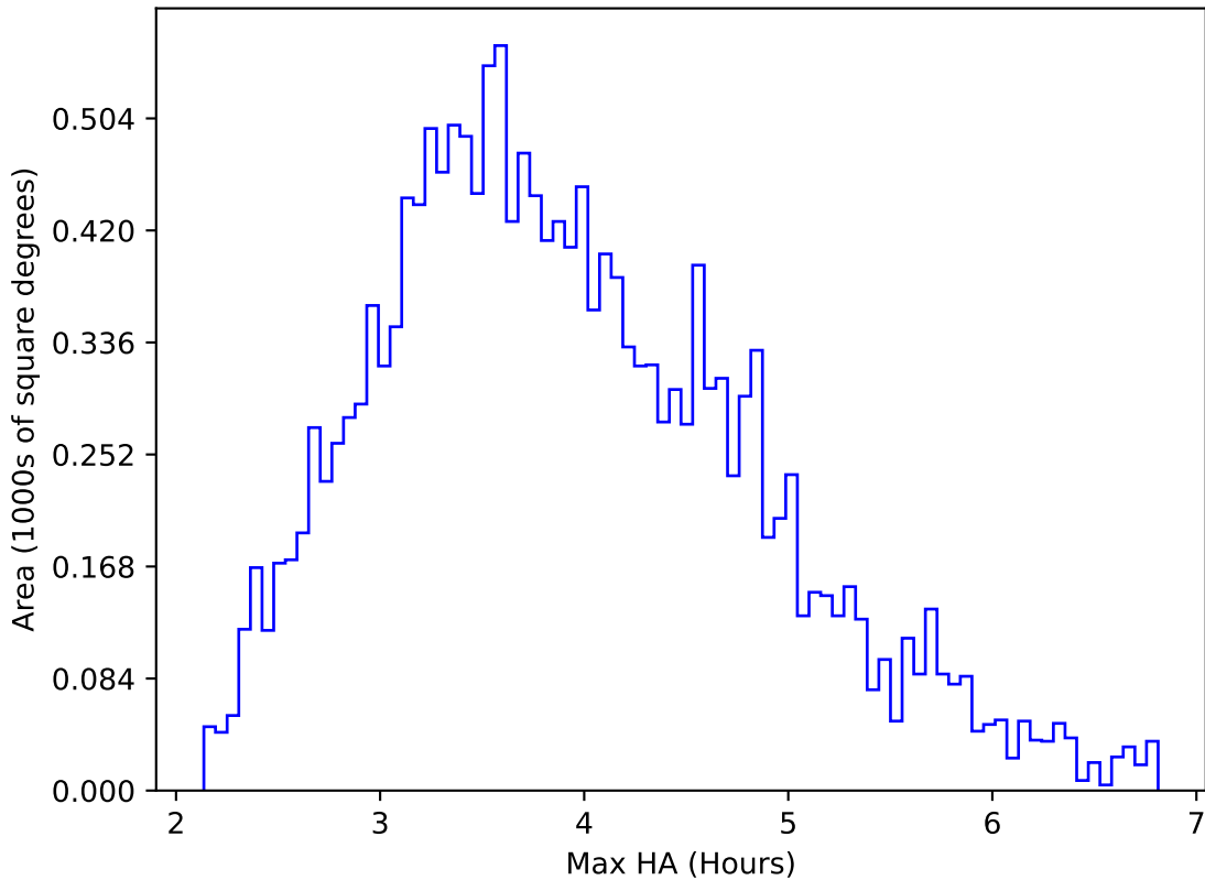
roll_pause_mjdp0_v3.4_10yrs WFD u band: Max HA
