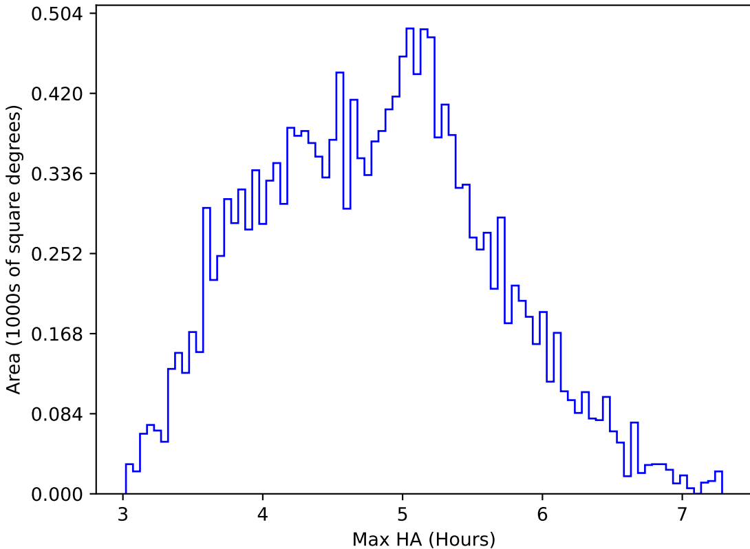
roll_pause_mjdp0_v3.4_10yrs WFD i band: Max HA
