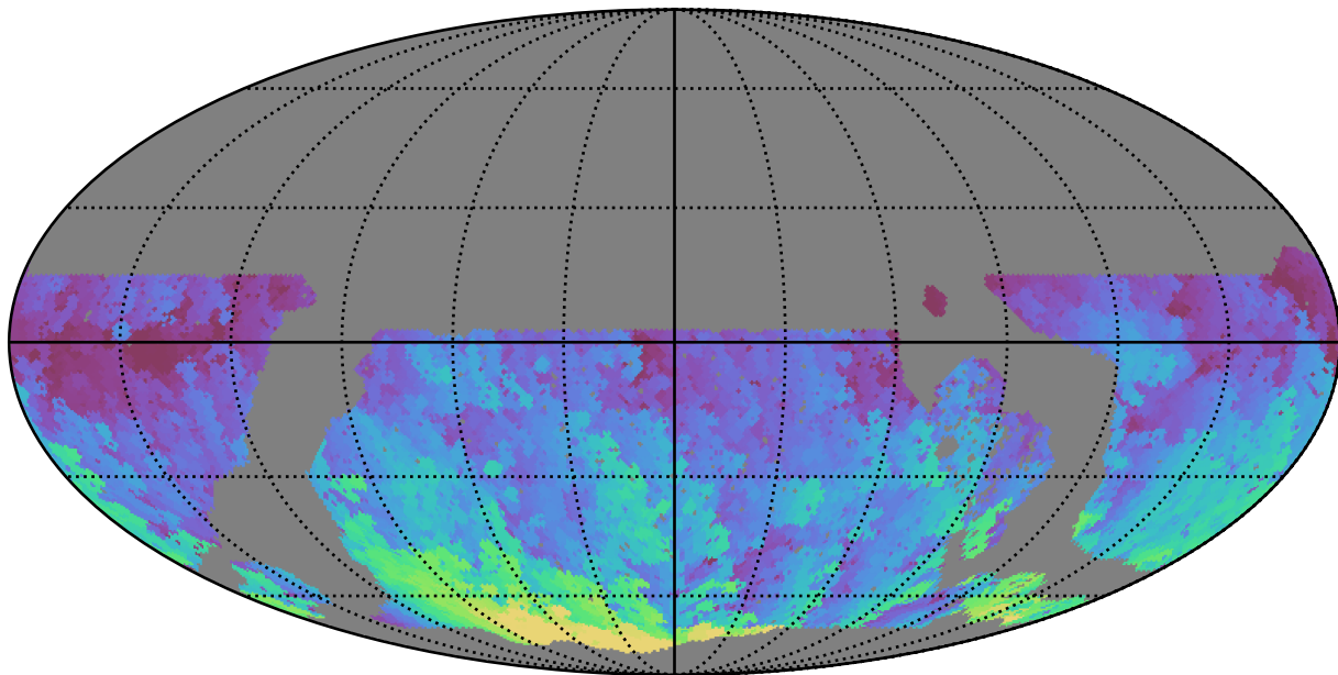
roll_pause_mjdp0_v3.4_10yrs WFD g band: Max HA
