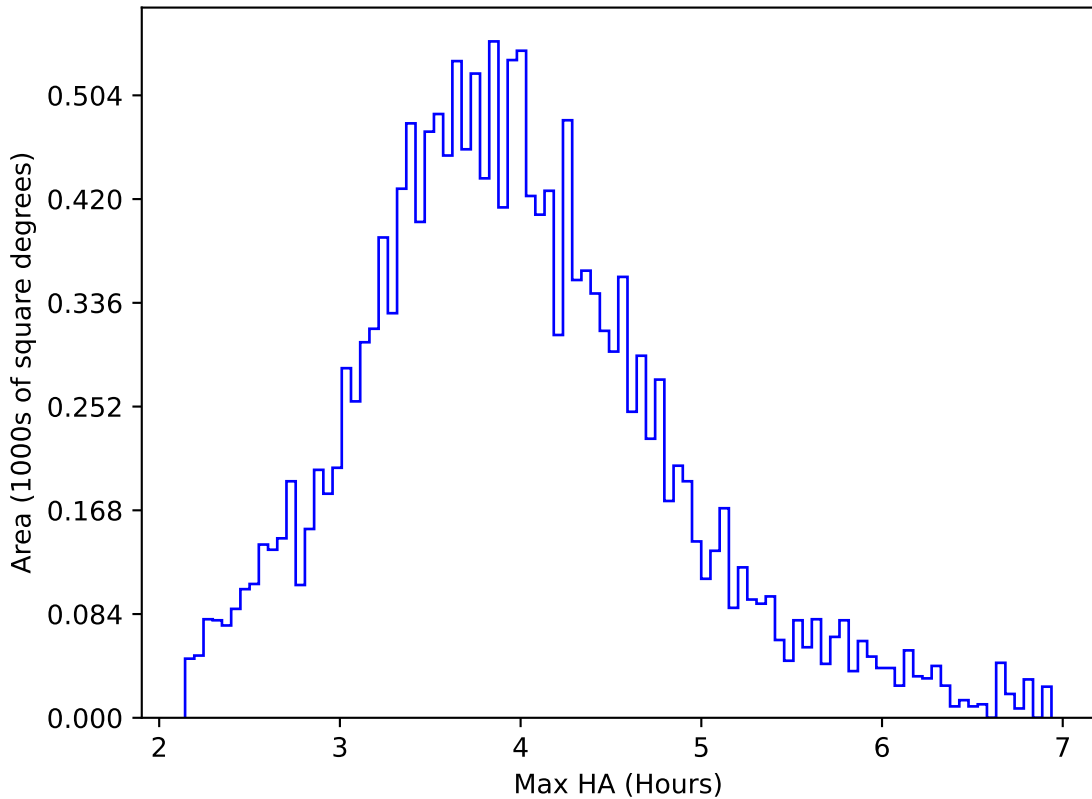
roll_pause_mjdp0_v3.4_10yrs WFD g band: Max HA
