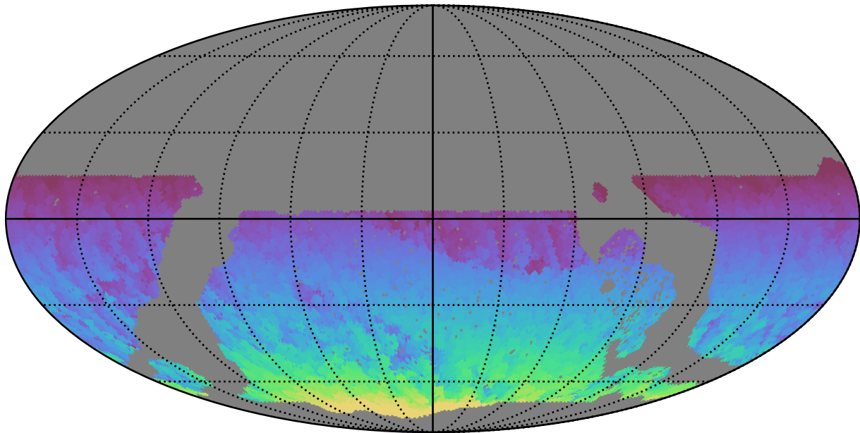
roll_pause_mjdp0_v3.4_10yrs WFD all bands: Max HA
