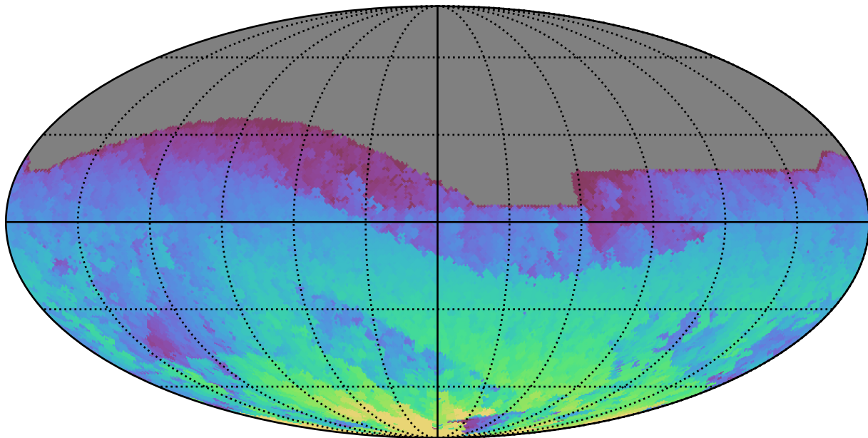
roll_pause_mjdp0_v3.4_10yrs All sky z band: Max HA
