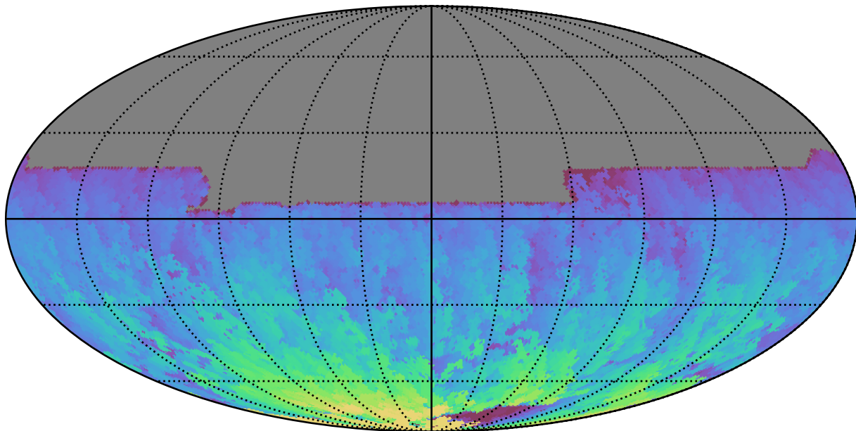
roll_pause_mjdp0_v3.4_10yrs All sky y band: Max HA
