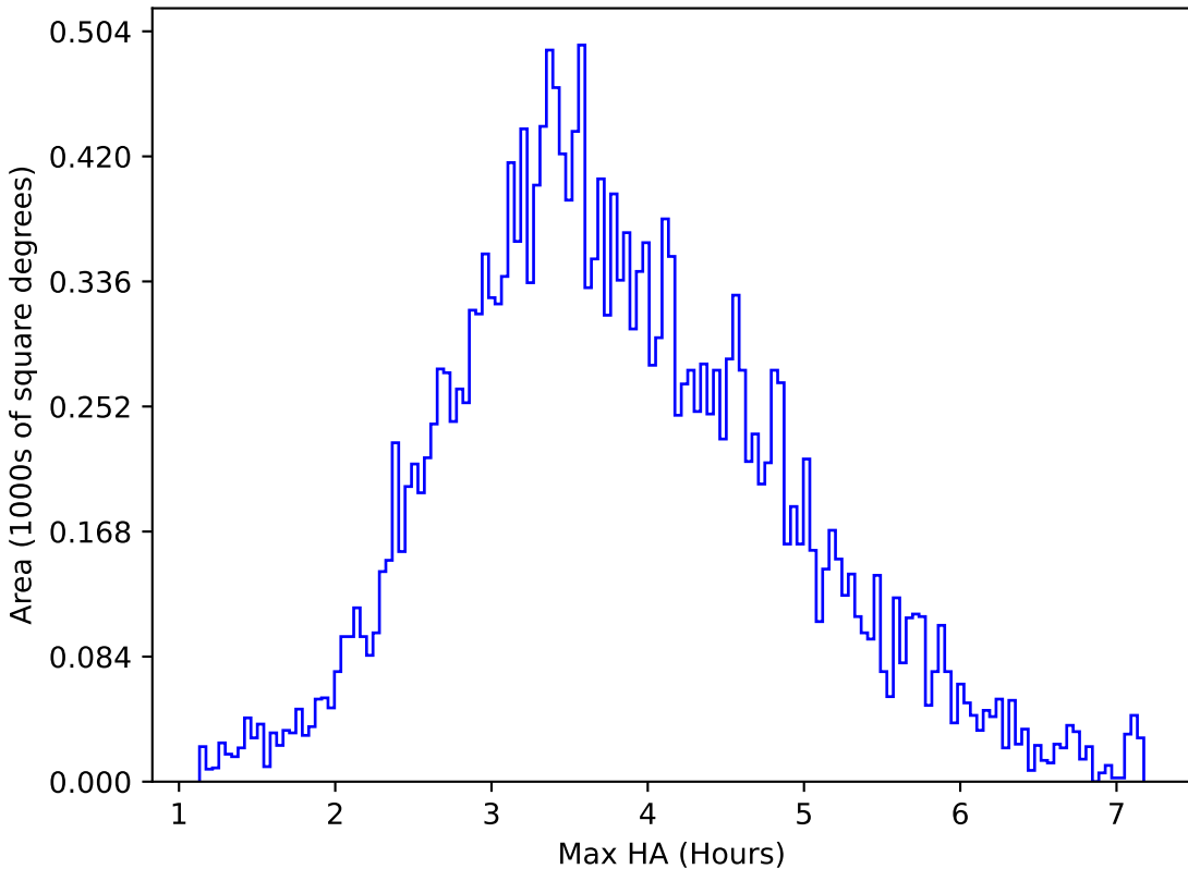
roll_pause_mjdp0_v3.4_10yrs All sky u band: Max HA
