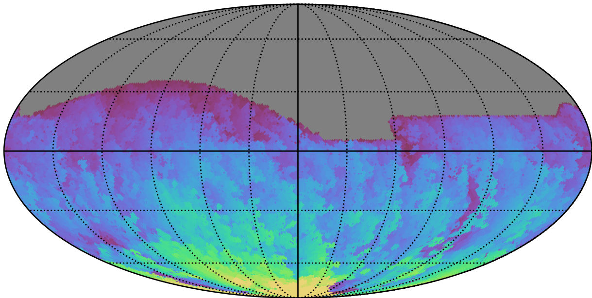
roll_pause_mjdp0_v3.4_10yrs All sky r band: Max HA
