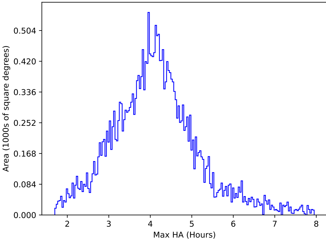
roll_pause_mjdp0_v3.4_10yrs All sky r band: Max HA
