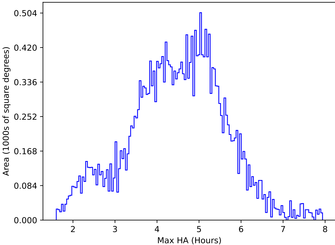
roll_pause_mjdp0_v3.4_10yrs All sky i band: Max HA
