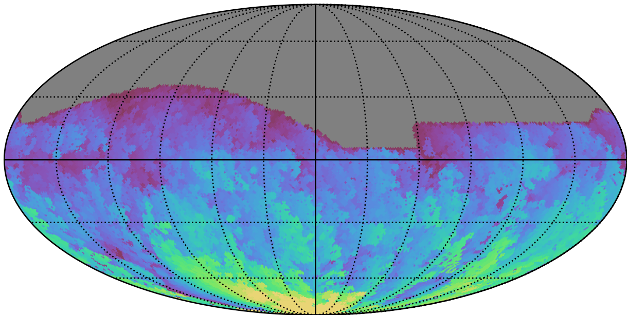
roll_pause_mjdp0_v3.4_10yrs All sky g band: Max HA
