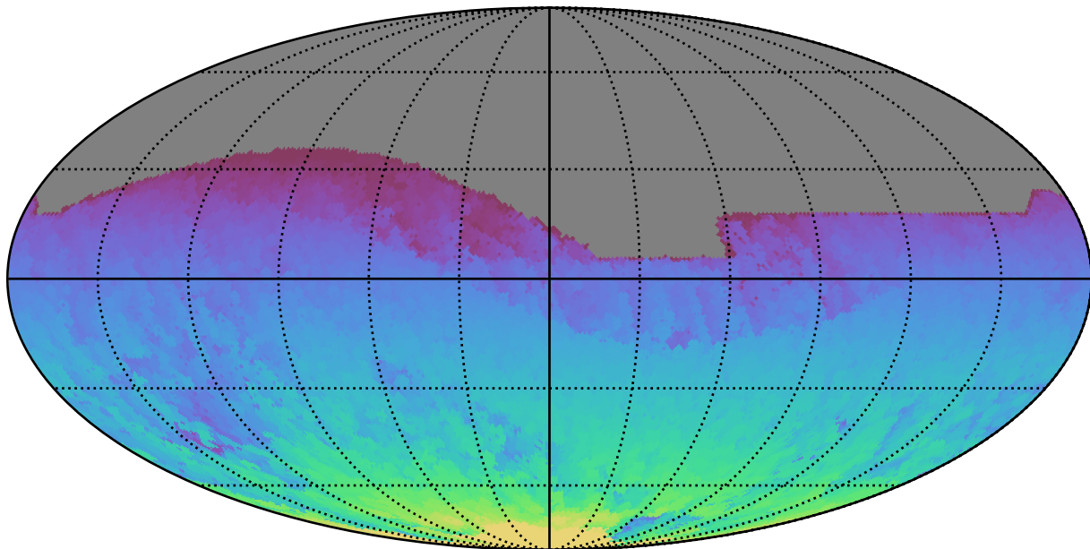
roll_pause_mjdp0_v3.4_10yrs All sky all bands: Max HA
