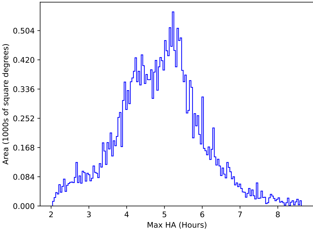
roll_pause_mjdp0_v3.4_10yrs All sky all bands: Max HA
