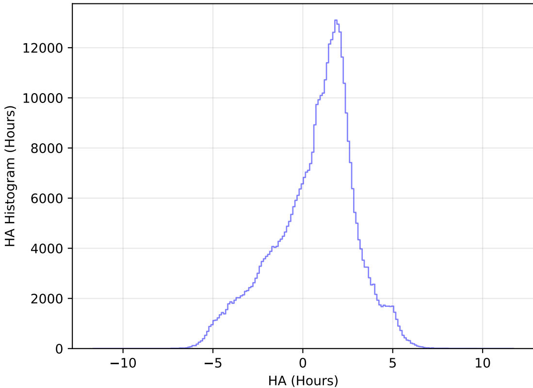
roll_pause_mjdp0_v3.4_10yrs WFD z band: HA Histogram
