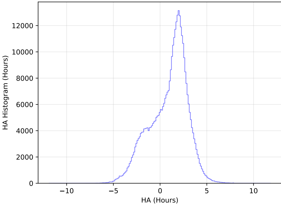
roll_pause_mjdp0_v3.4_10yrs WFD y band: HA Histogram
