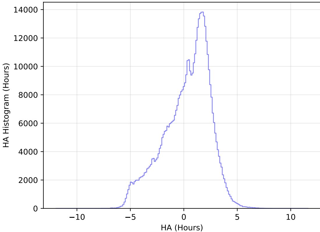
roll_pause_mjdp0_v3.4_10yrs WFD r band: HA Histogram
