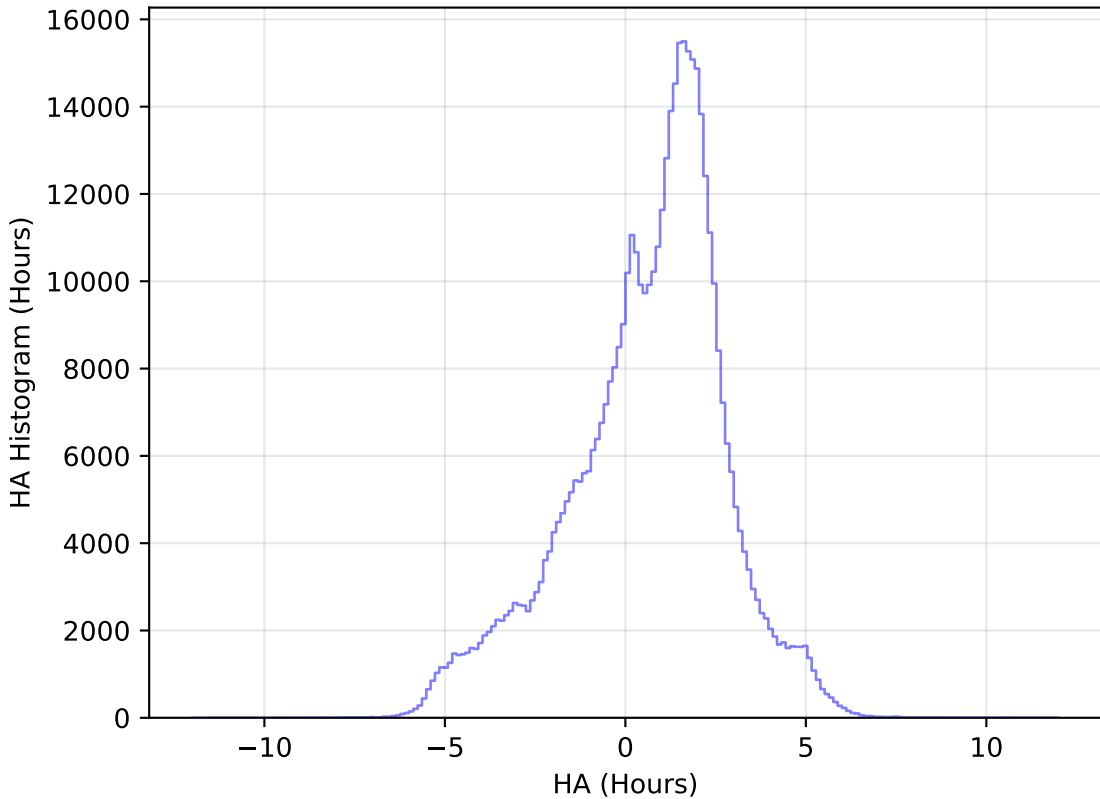
roll_pause_mjdp0_v3.4_10yrs WFD i band: HA Histogram
