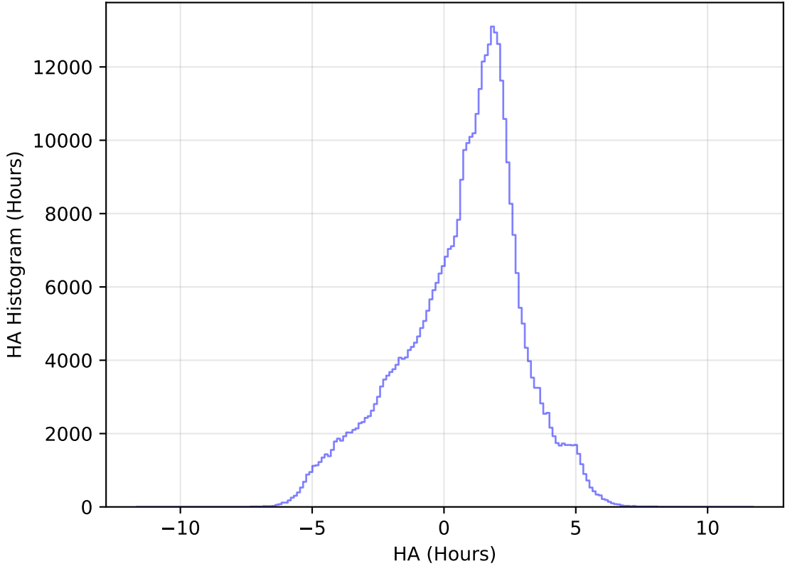
roll_pause_mjdp0_v3.4_10yrs All sky z band: HA Histogram
