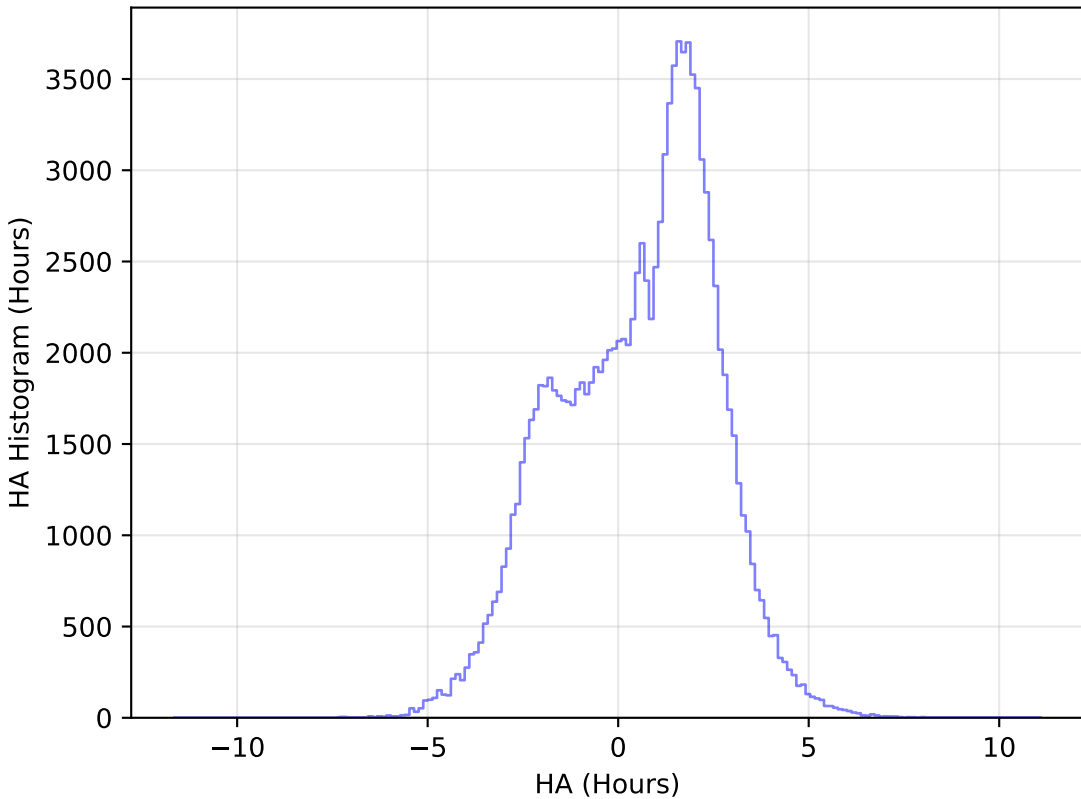
roll_pause_mjdp0_v3.4_10yrs All sky u band: HA Histogram
