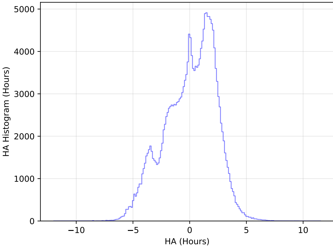
roll_pause_mjdp0_v3.4_10yrs All sky g band: HA Histogram
