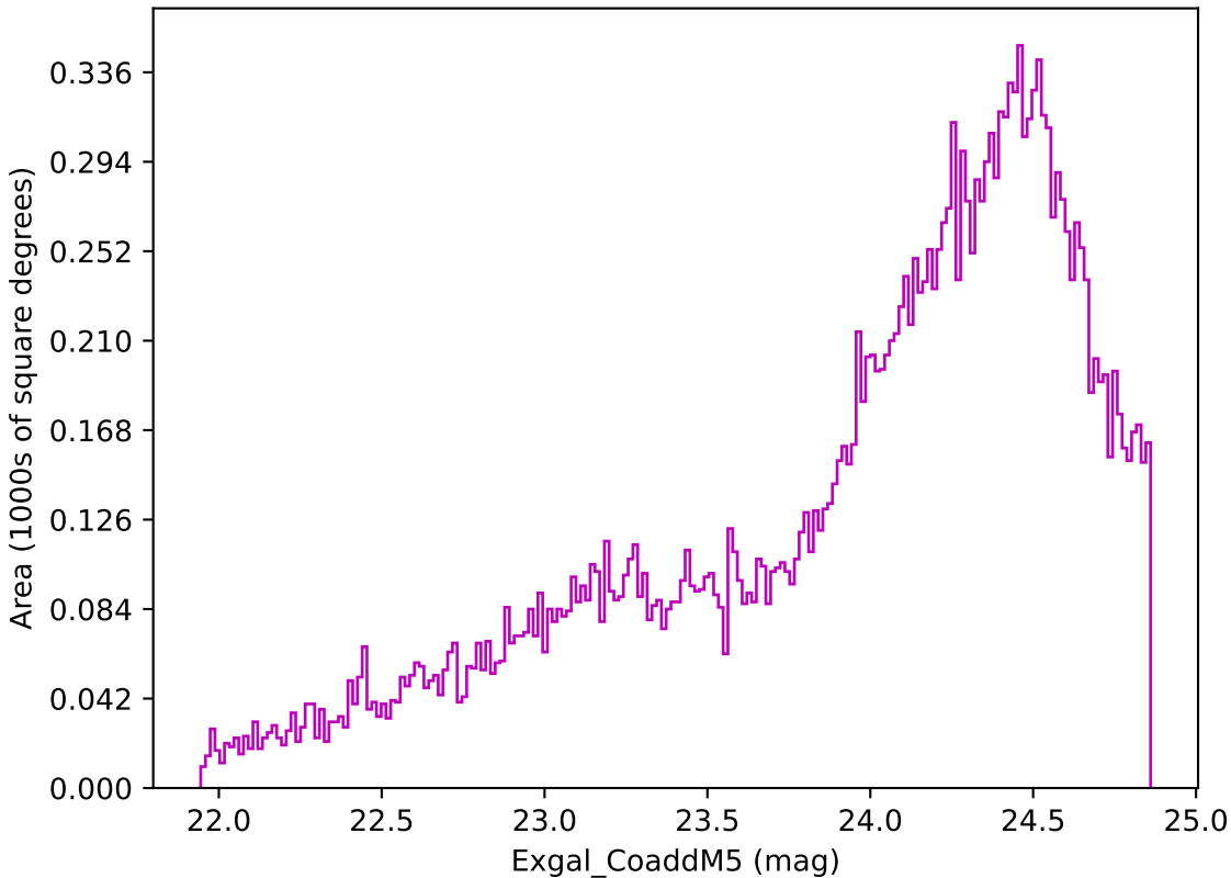
roll_pause_mjdp0_v3.4_10yrs Yr 3-4 z band: Exgal_CoaddM5
