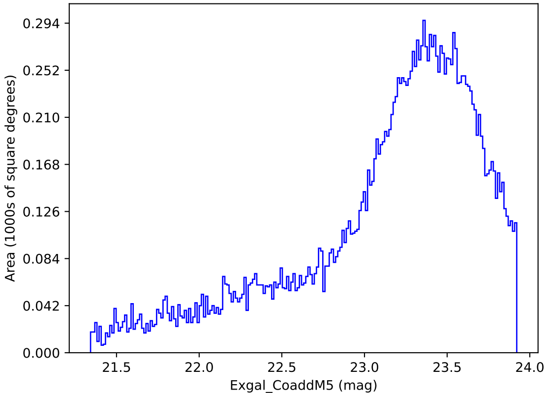
roll_pause_mjdp0_v3.4_10yrs Yr 3-4 y band: Exgal_CoaddM5
