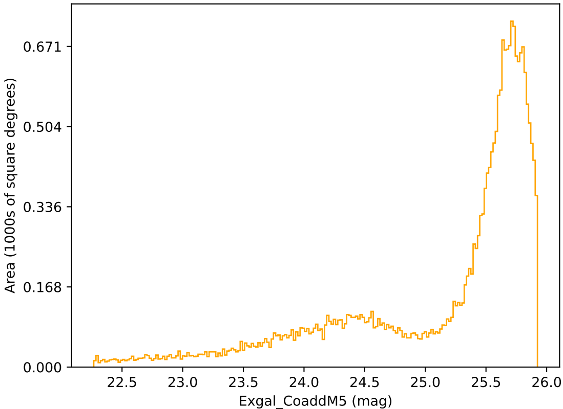
roll_pause_mjdp0_v3.4_10yrs Yr 1 r band: Exgal_CoaddM5
