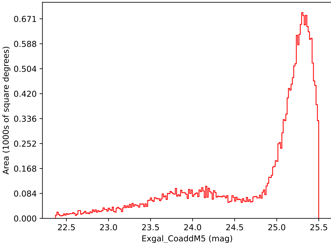
roll_pause_mjdp0_v3.4_10yrs Yr 1 i band: Exgal_CoaddM5
