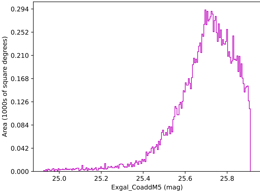
roll_pause_mjdp0_v3.4_10yrs WFD z band: Exgal_CoaddM5
