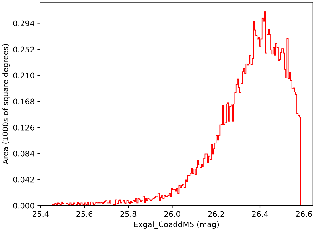
roll_pause_mjdp0_v3.4_10yrs WFD i band: Exgal_CoaddM5
