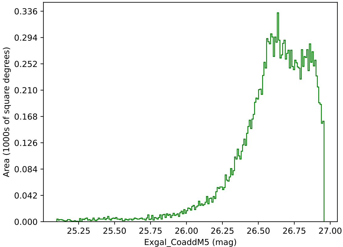
roll_pause_mjdp0_v3.4_10yrs WFD g band: Exgal_CoaddM5
