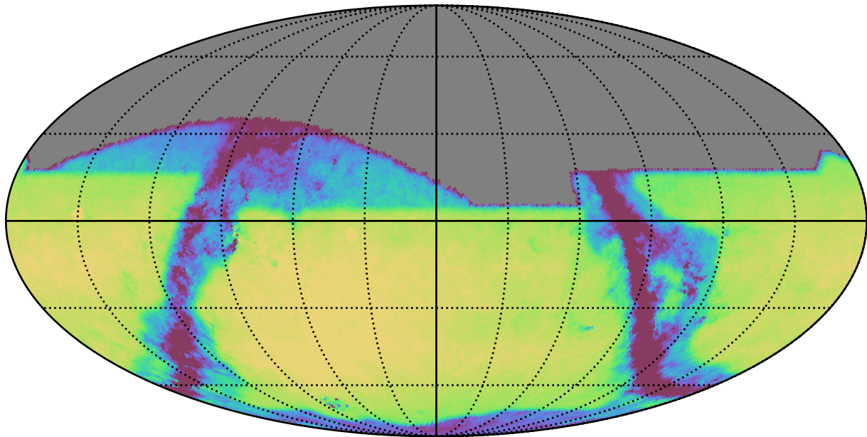
roll_pause_mjdp0_v3.4_10yrs All sky z band: Exgal_CoaddM5
