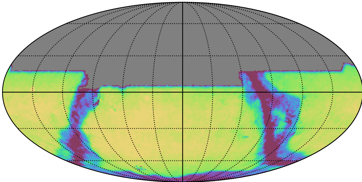
roll_pause_mjdp0_v3.4_10yrs All sky y band: Exgal_CoaddM5
