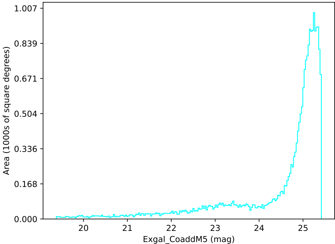
roll_pause_mjdp0_v3.4_10yrs All sky u band: Exgal_CoaddM5
