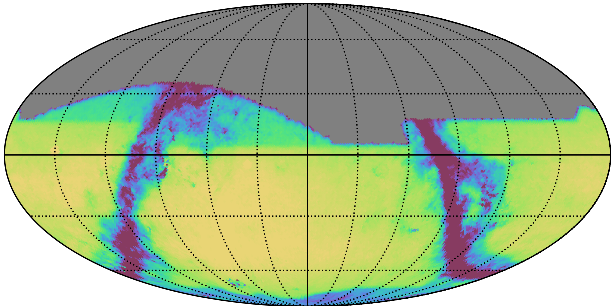
roll_pause_mjdp0_v3.4_10yrs All sky r band: Exgal_CoaddM5
