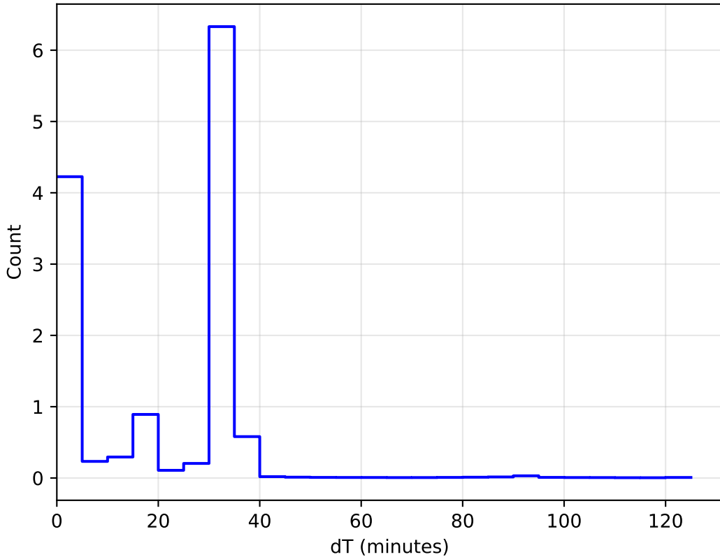
roll_pause_mjdp0_v3.4_10yrs All sky: DeltaT Histogram
