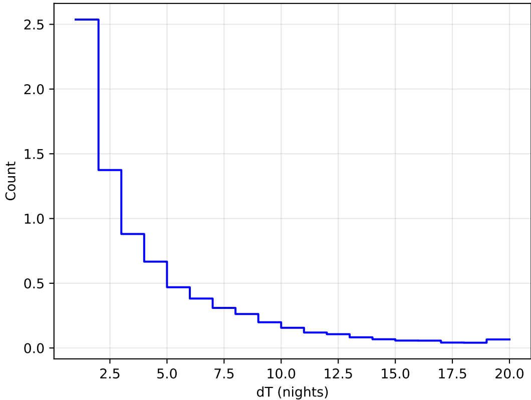
roll_pause_mjdp0_v3.4_10yrs WFD all bands: DeltaNight Histogram 1e6
