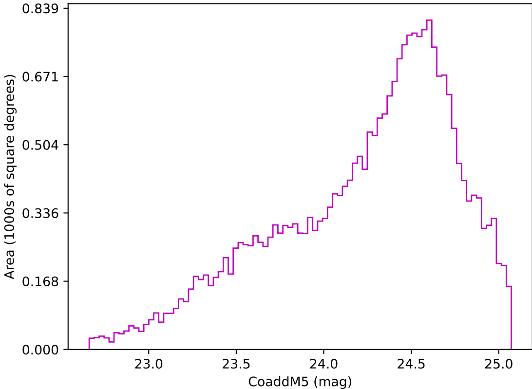
roll_pause_mjdp0_v3.4_10yrs Yr 3-4 z band: CoaddM5
