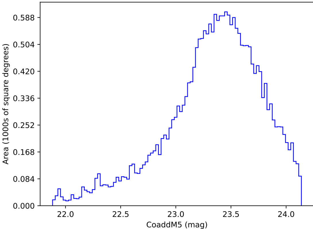
roll_pause_mjdp0_v3.4_10yrs Yr 3-4 y band: CoaddM5
