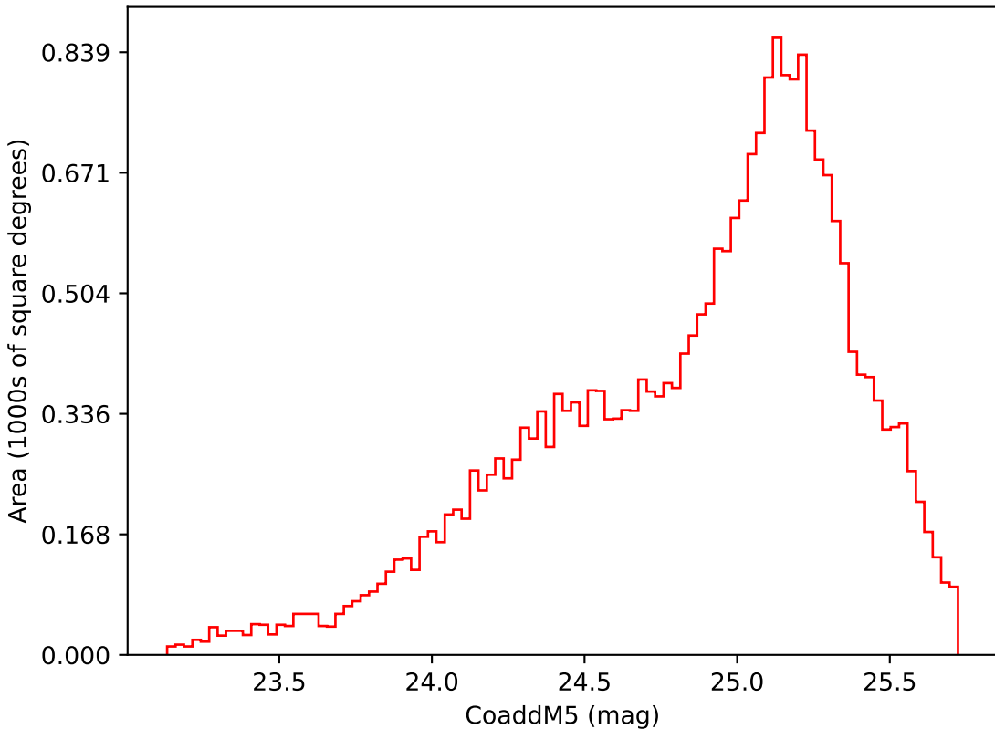
roll_pause_mjdp0_v3.4_10yrs Yr 3-4 i band: CoaddM5
