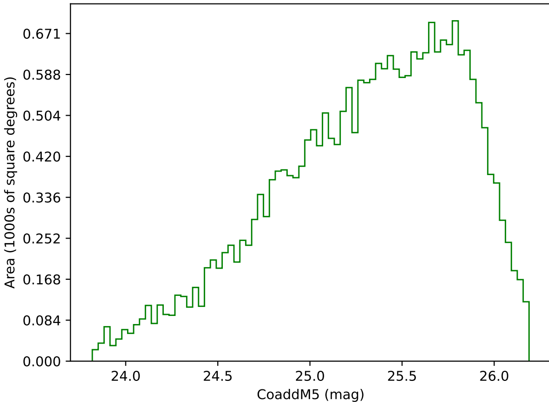
roll_pause_mjdp0_v3.4_10yrs Yr 3-4 g band: CoaddM5
