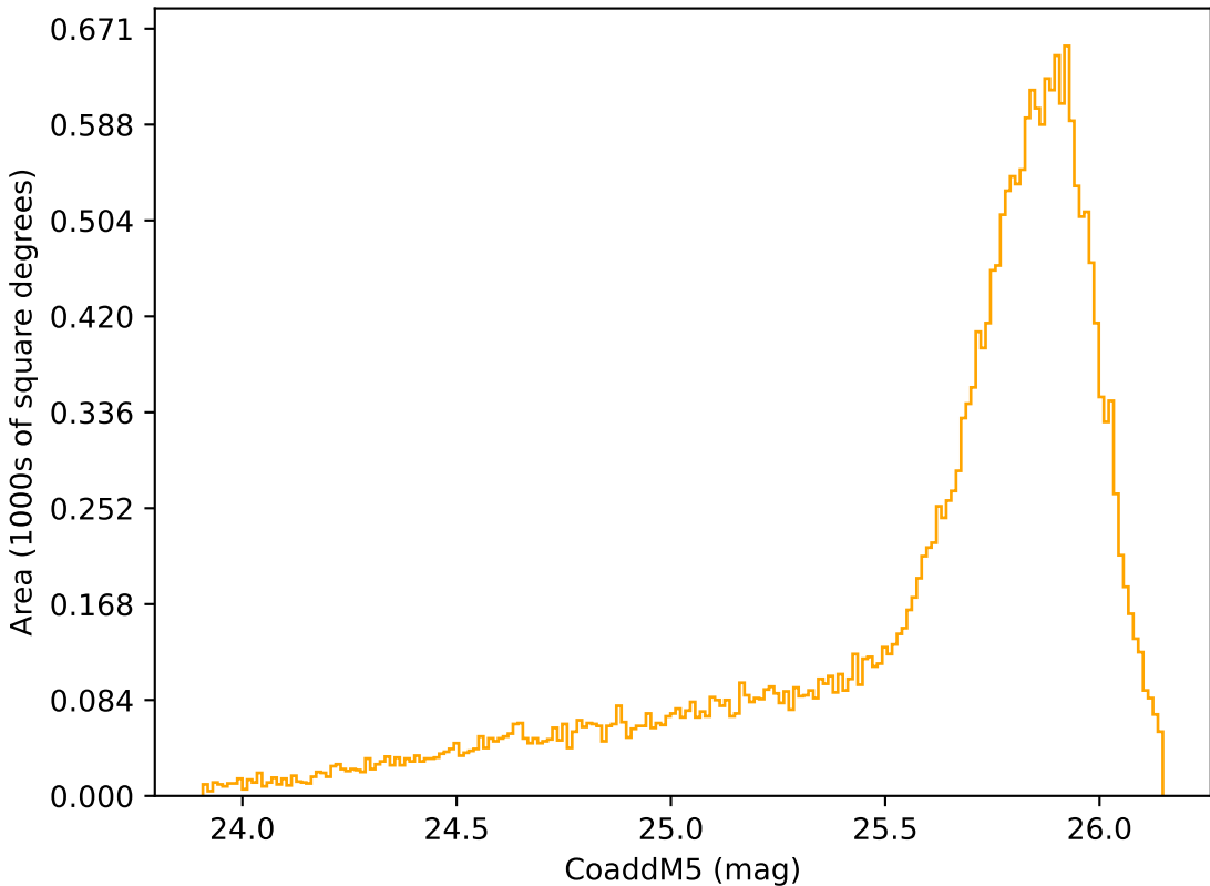
roll_pause_mjdp0_v3.4_10yrs Yr 1 r band: CoaddM5
