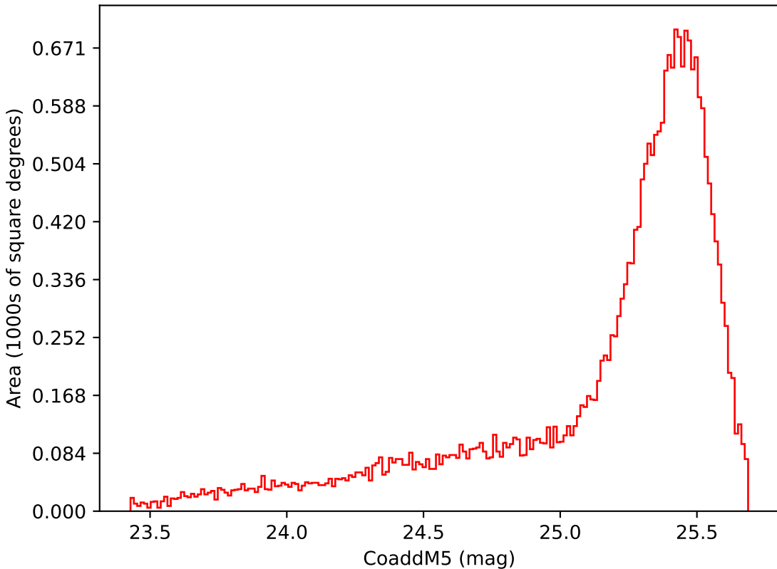
roll_pause_mjdp0_v3.4_10yrs Yr 1 i band: CoaddM5
