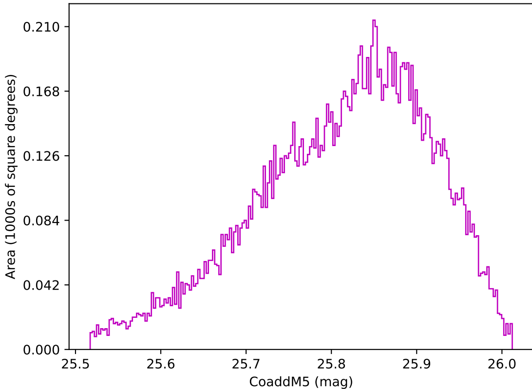
roll_pause_mjdp0_v3.4_10yrs WFD z band: CoaddM5
